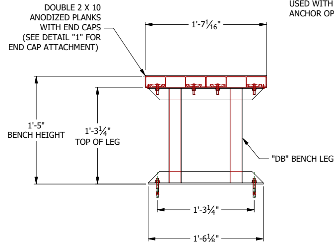
CONCRETE ANCHOR OPTION SEE DETAIL "4" (CONCRETE PAD REQUIRED BY OTHERS)
