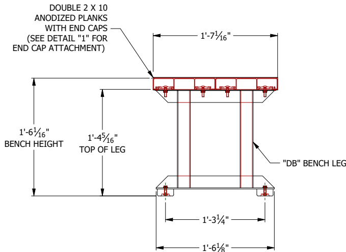
RUBBER FOOT PAD OPTION SEE DETAIL "3" (CONCRETE ANCHORS NOT USED)
